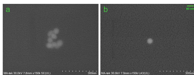
Figure 2: Comparing the differences in results obtained from SEM measurements of nanoparticles in liquid environments, the images present in a 2D format, unable to clearly display surface morphology. BSE imaging is relatively clearer than SE imaging. a is showing the SE image and b is showing the BSE image. The experiment employs a 30 kV acceleration voltage. 60 nm gold nanoparticles.
